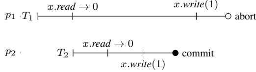
Figure 1. An illustration of the difficulty of ensuring local progress. The scenario can repeat infinitely many times preventing transaction T_1 from ever committing.
